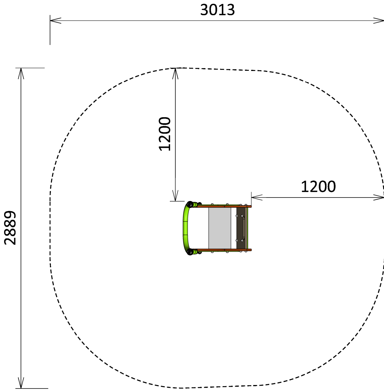
ACCESSIBLE DIPPER ROCKER (SE-71)
