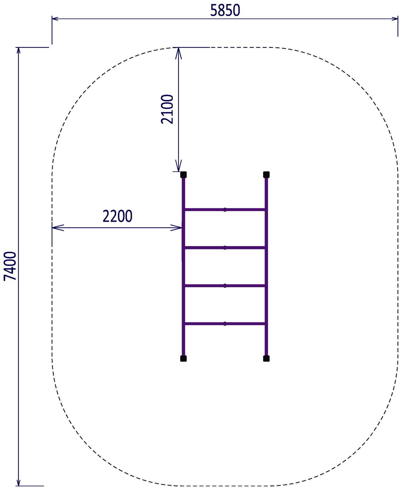
NINJA GRIP TRAVERSE 2300 HIGH
